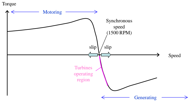
Induction generator torque-speed curve
